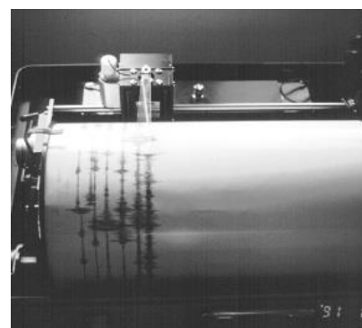
Figure 20 - Seismograph trace from Mount Pinatubo
