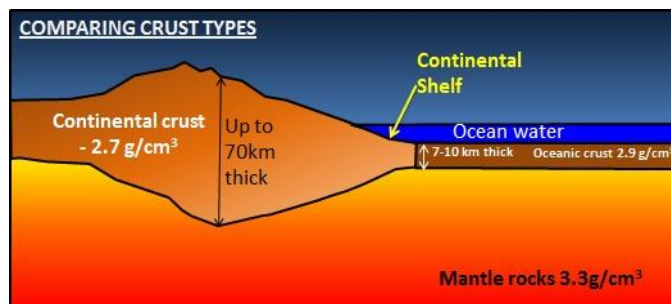
Figure 5 Contrasts between Oceanic and continental crust
