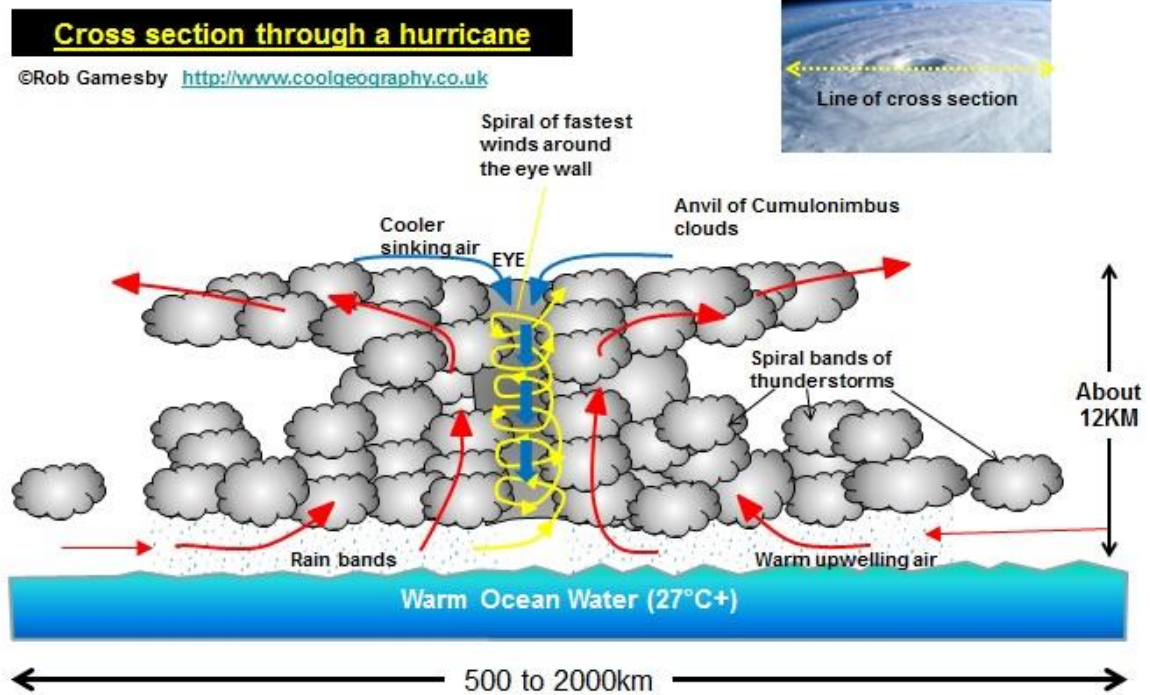
Figure 23 - a cross section through a tropical storm
