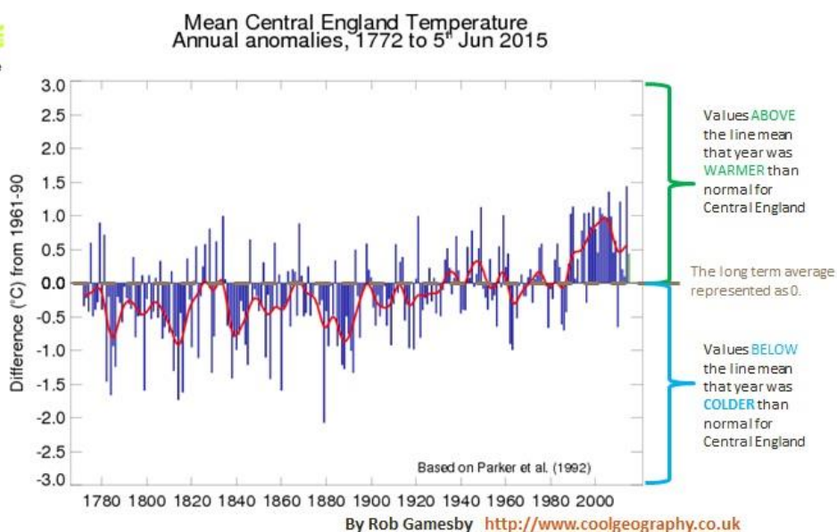
Figure 37 - Temperature records for Central England
