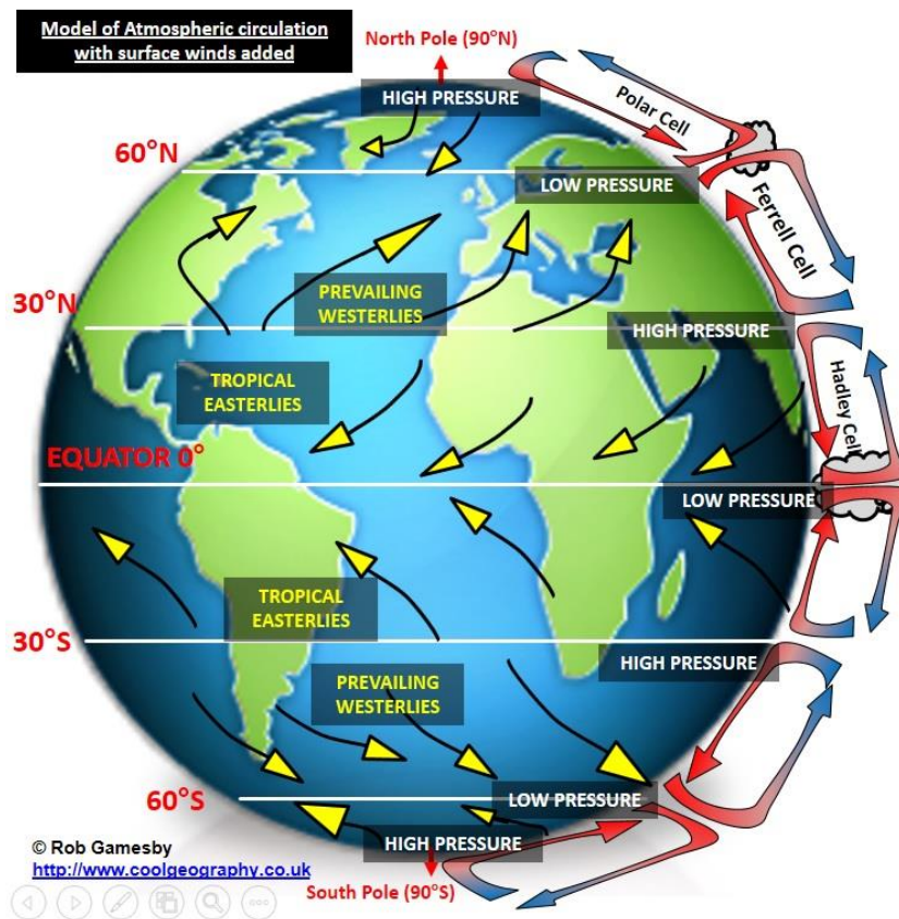
Figure 22 - A model of atmospheric circulation
