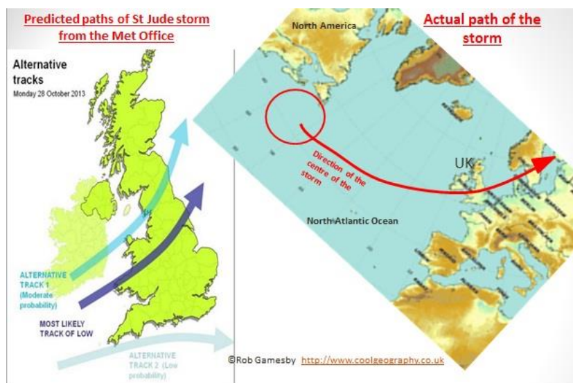
Figure 38 - the path of the St Jude Storm
