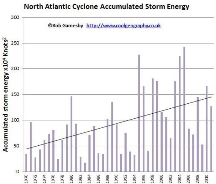
Figure 26 - Tropical storm totals
