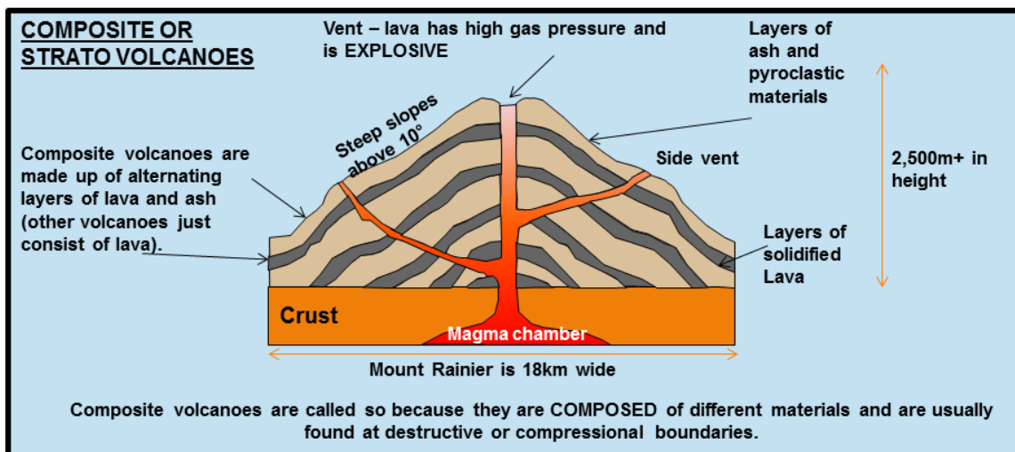
Figure 12 - Strato volcanoes
