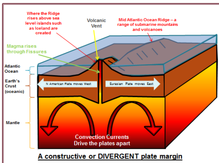
Figure 7 A constructive plate margin
