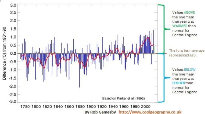
Mean Central England Temperature Annual anomalies, 1772 to 5 th Jun 2015
