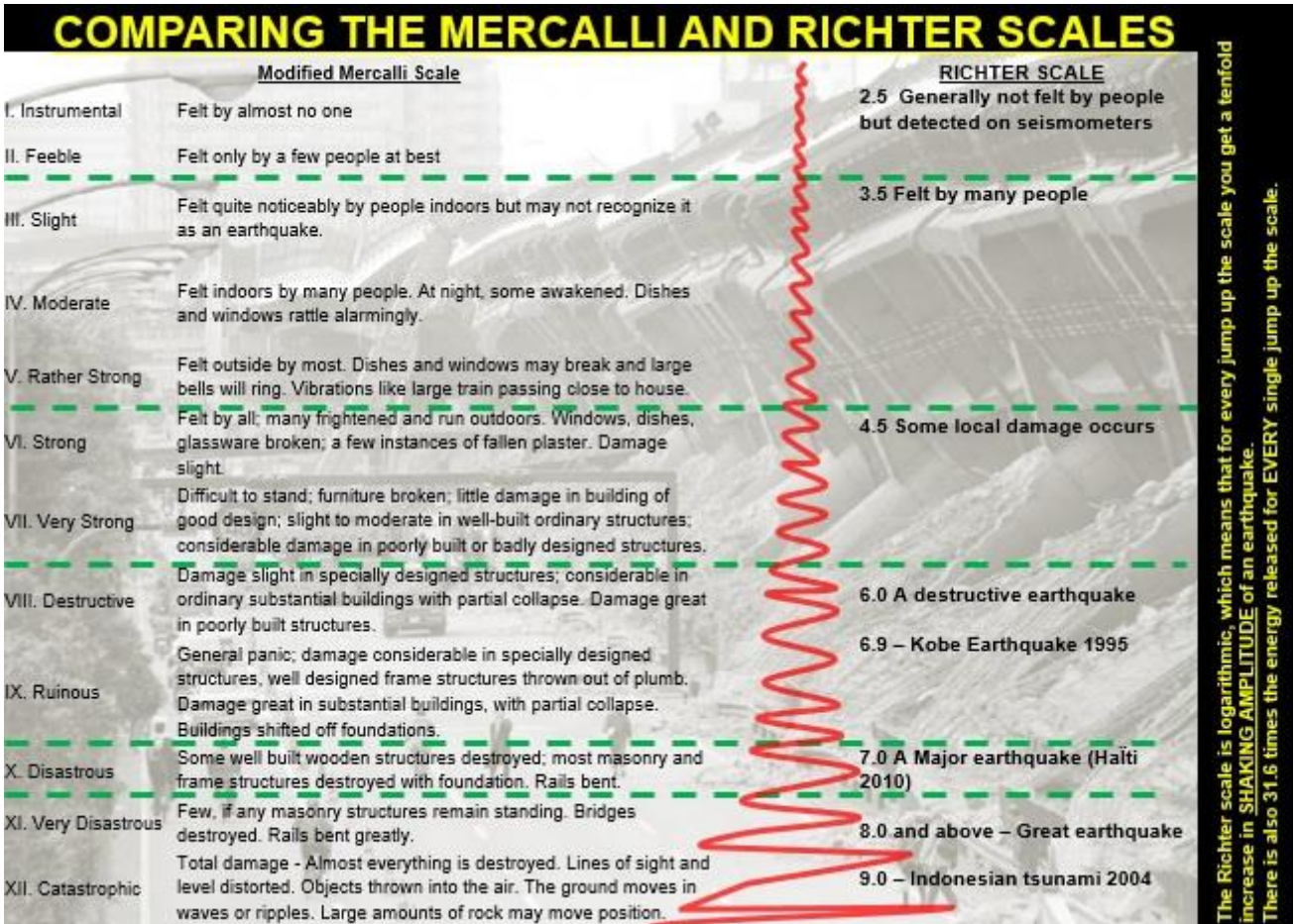
Figure 2 The Richter and Mercalli Scales
