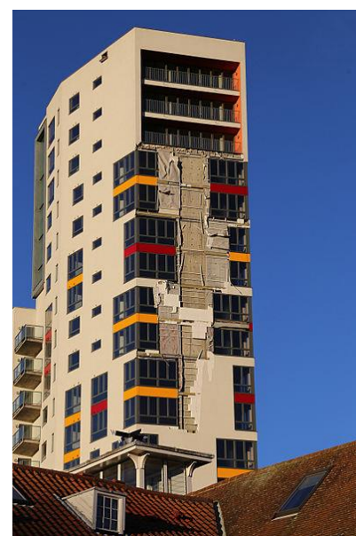
Figure 39 - Damage to cladding of a building in Ipswich - By Steven James Fosdick on Wikimedia
