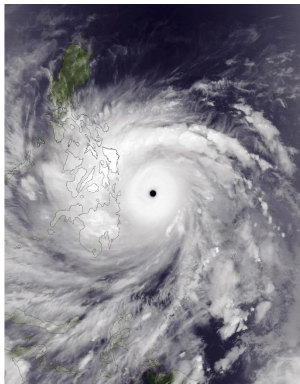
Figure 30 - NASA image of Typhoon Haiyan By NASA, LAADS Web,
