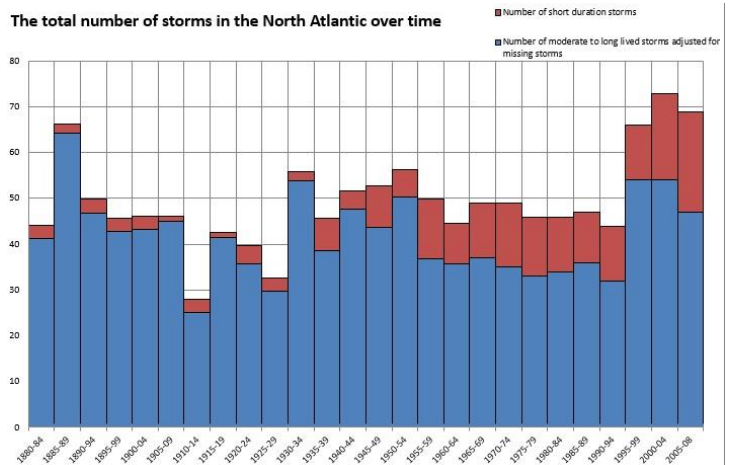
Figure 26 - Tropical storm totals
