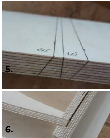
These pictures show how I worked out the angles to cut the ends of the plywood at from my scale drawing.
