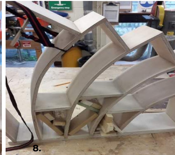
Then I cut the shelves and used the disc sander to create the angles so they fitted in between the upright pieces. I used PVA glue to attach them in place. Using a wet cloth and sand paper I cleaned up excess glue and sanded all surfaces to give a smooth finish.
